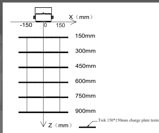
Test bearing chart of air blower
