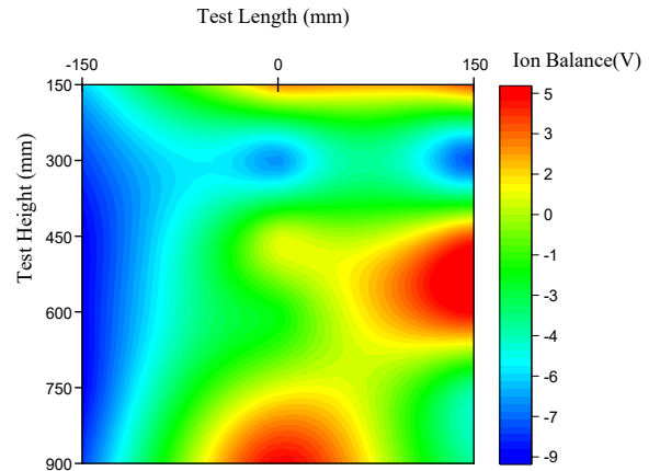
Ion balance distribution diagram of AP-DJ2811
