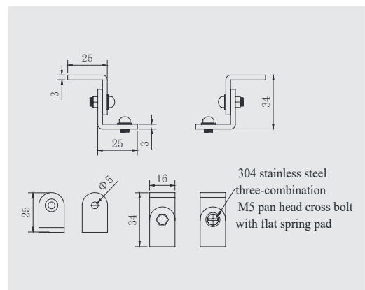
Mounting bracket size drawing
